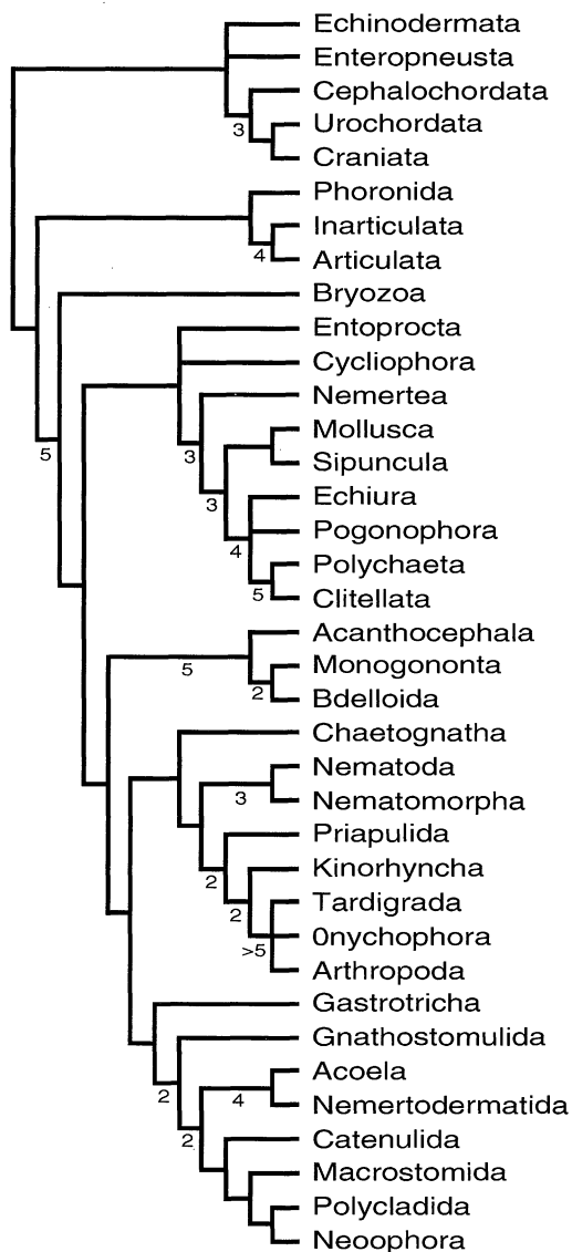
FIGURE 3. Strict consensus of 16 trees of 455 steps (consistency index = 0.466; retention index = 0.701) based on the morphological data of Zrzavý et al. (1998). Bremer support values >1 are indicated.
