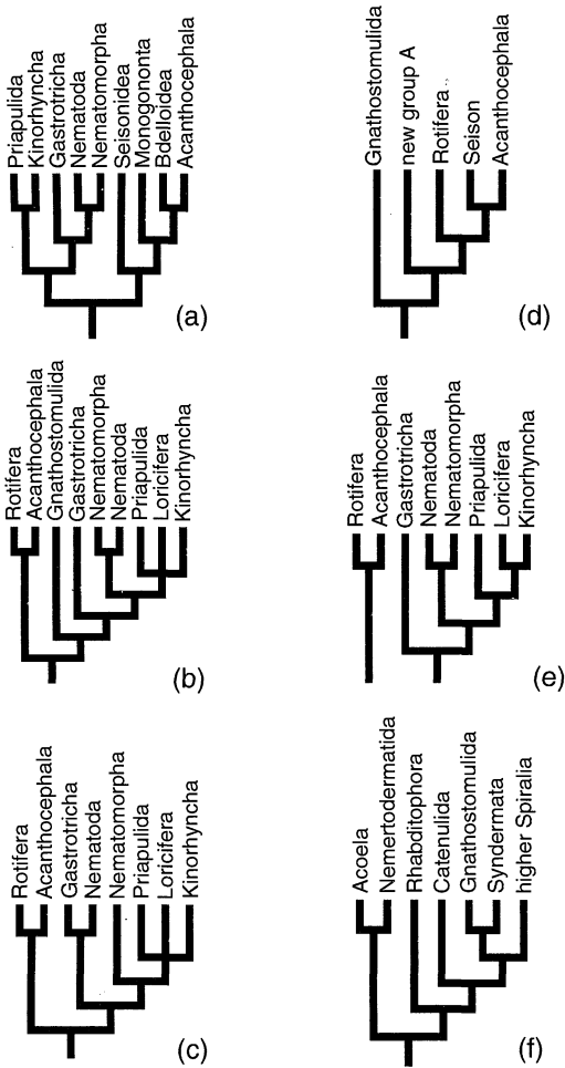
FIGURE 1. Phylogenetic hypotheses for different platyzoan taxa. (a) Lorenzen (1985). (b) Wallace et al. (1995, 1996). (c) Neuhaus et al. (1996). (d) Ahlrichs (1995, 1997); (e) Nielsen (1995); Nielsen et al. (1996). (f) Haszprunar (1996).
