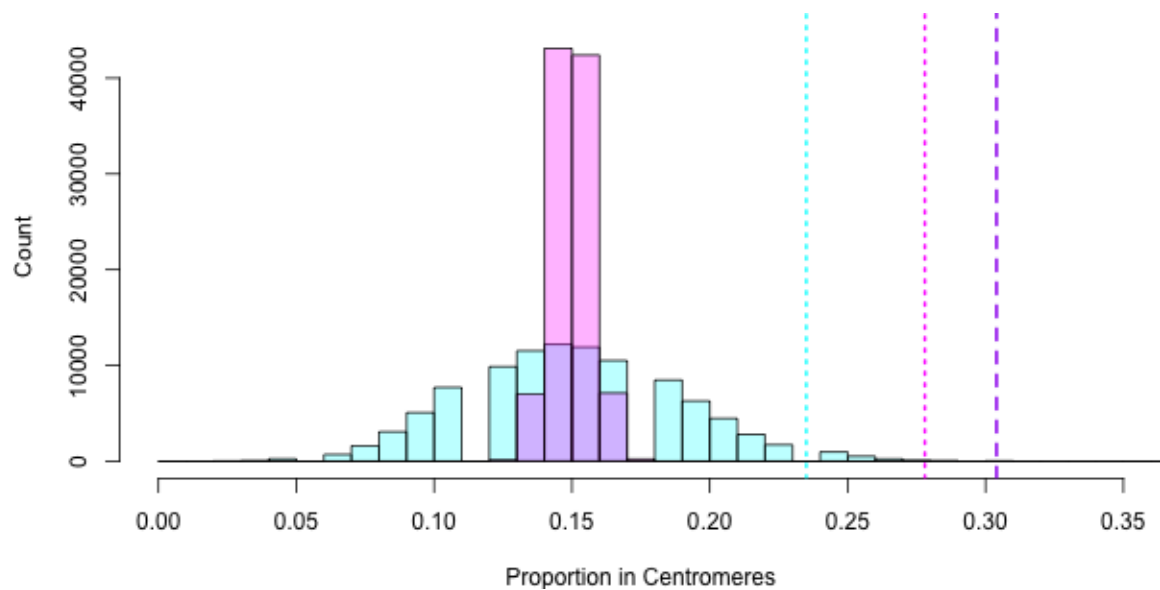
Supplementary Figure 4.13: Islands and sweeps are over-represented in the centromeres. X-axis is the simulated proportion of islands and sweeps in the centromeres. Y-axis is the number of simulations that fell within a given position. Pink bars show values for sweeps (N=2,960), blue bars for islands (N=83), and the purple indicates where they overlap. Vertical lines are the empirical estimates of the proportions within centromeres. Purple dashed line shows proportion of total windows that are in centromeres for both islands and sweeps. Pink dotted line shows proportion of total regions that are in centromeres for sweeps. Blue dotted line shows proportions of total regions that are in centromeres for islands.
