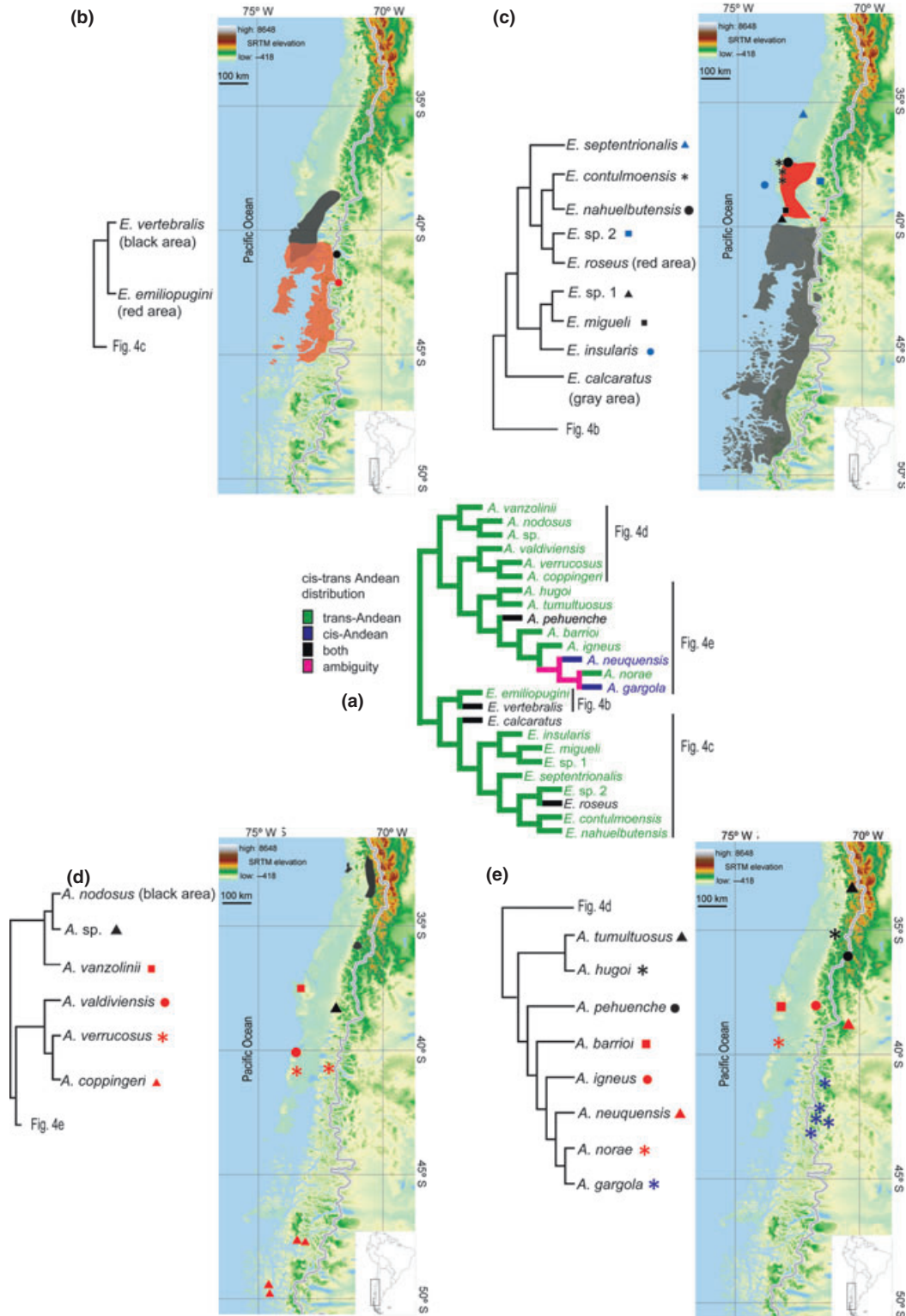
Fig. 4. Distribution of the species of Alsodes and Eupsophus (b–e), and optimization of those distributions according to cis - and trans -Andean ranges (a) in one of the optimal cladograms (the ingroup topology is nearly constant in all analyses, with minor differences, irrelevant for our inferences). For the sake of clarity, Alsodes and Eupsophus clades are divided into two clades each (b–e). See Appendix S4 for the literature sources of species distributions, and for specific considerations for the optimization of the cis - and trans -Andean distribution. Among species not sampled (besides those known only from type material and not collected since original description) are A. montanus and A. kaweshkari , both with trans -Andean distribution (Formas et al., 1998; Correa et al., 2008).
